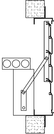
Model 1307 Front Flange Mount (shown blades closed)
