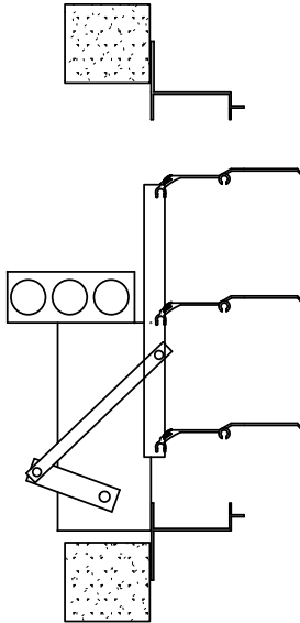
Model 1305 Flange Mount (shown blades open)
